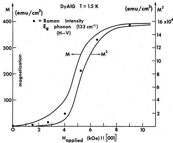
FIG. 7. Observed Raman intensity due to the E_g ( 133 \text{ cm}^{-1} ) phonon as a function of the applied magnetic field. For the H - V polarizations, Raman scattering from the E_g phonons is forbidden for crystals of O_h and C_{4h} point groups (see Table IV). The intensity at 9 kOe was normalized to 385 relative units (same scale as M ). The magnetization and the square of the magnetization versus applied field data were obtained from Ref. 18 and are shown here for comparison purposes.
