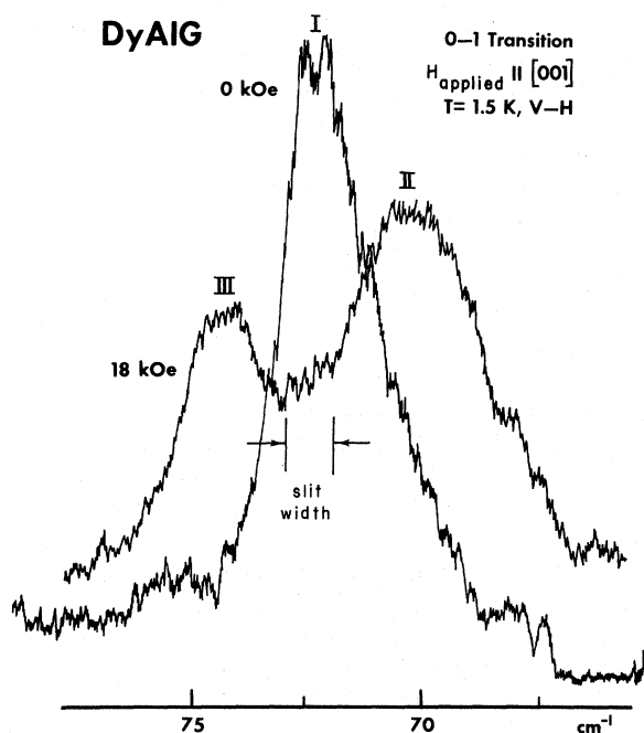
FIG. 2. Raman spectra of DyAlG at 1.5 K involving electronic transitions from the ground state 0 to the first excited state 1 of the {}^6H_{15/2} manifold. Peak I was observed with H_{app}=0 kOe, while peaks II and III were observed with H_{app}=18 kOe along [001]. The incident and scattered polarizations were V-H (see Fig. 1).
